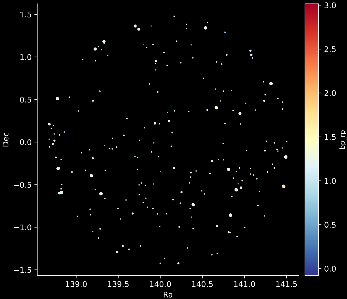
APOGEE DR17 Field: [171-52_MGA] Stars: 200
