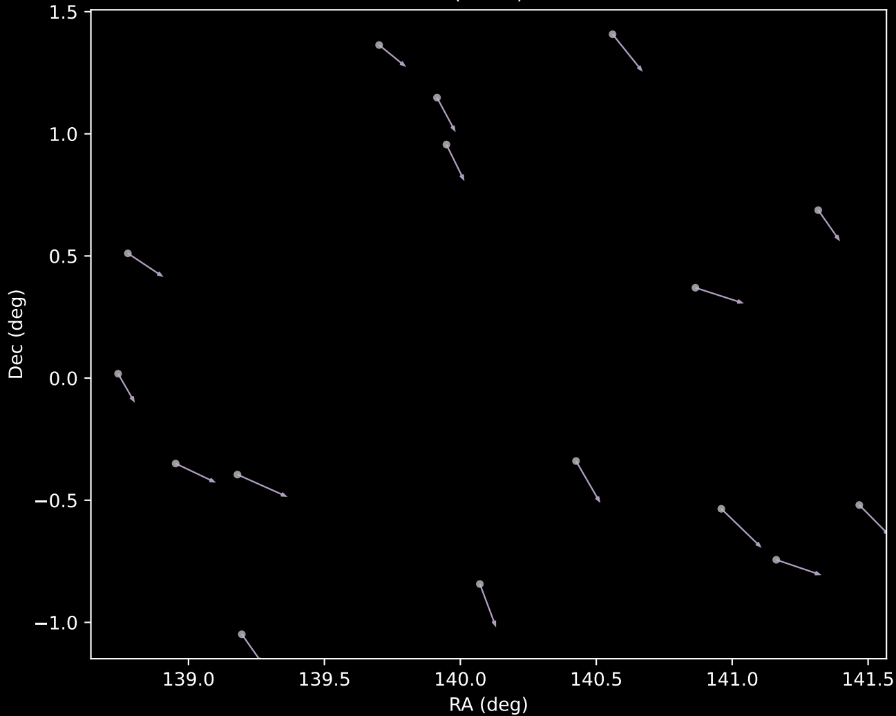
APOGEE DR17 Cluster 9 Proper Motion Vectors (n=16)
