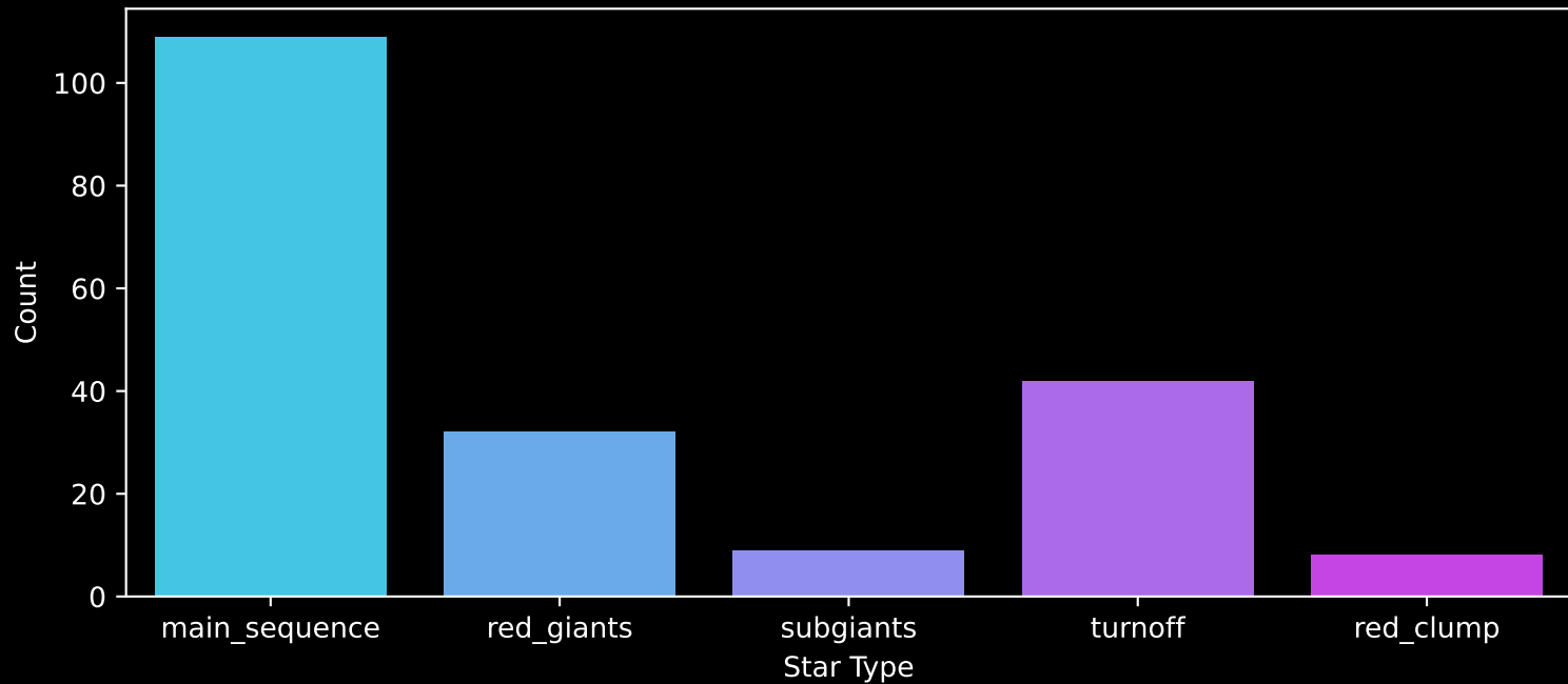
APOGEE DR17 Field: [171-52_MGA] Count plot of Star Type
