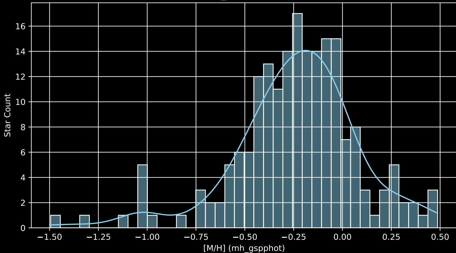
APOGEE DR17 Field: [171-52_MGA [M/H] (mh_gspphot) (n= 194)
