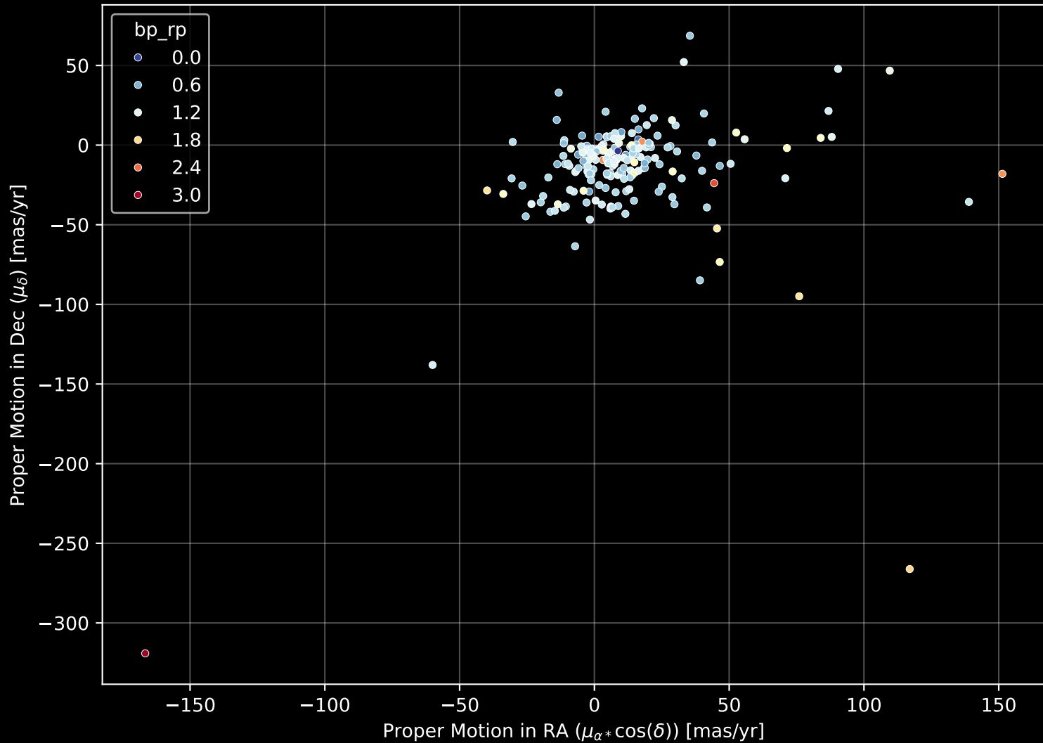
APOGEE DR17 Field: [171-52_MGA] Proper Motion Diagram (n= 200)
