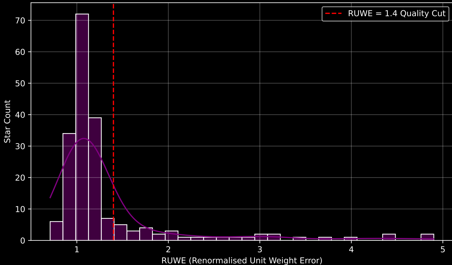
GAPOGEE DR17 Field [171-52_MGA] RUWE Distribution (n= 192)
