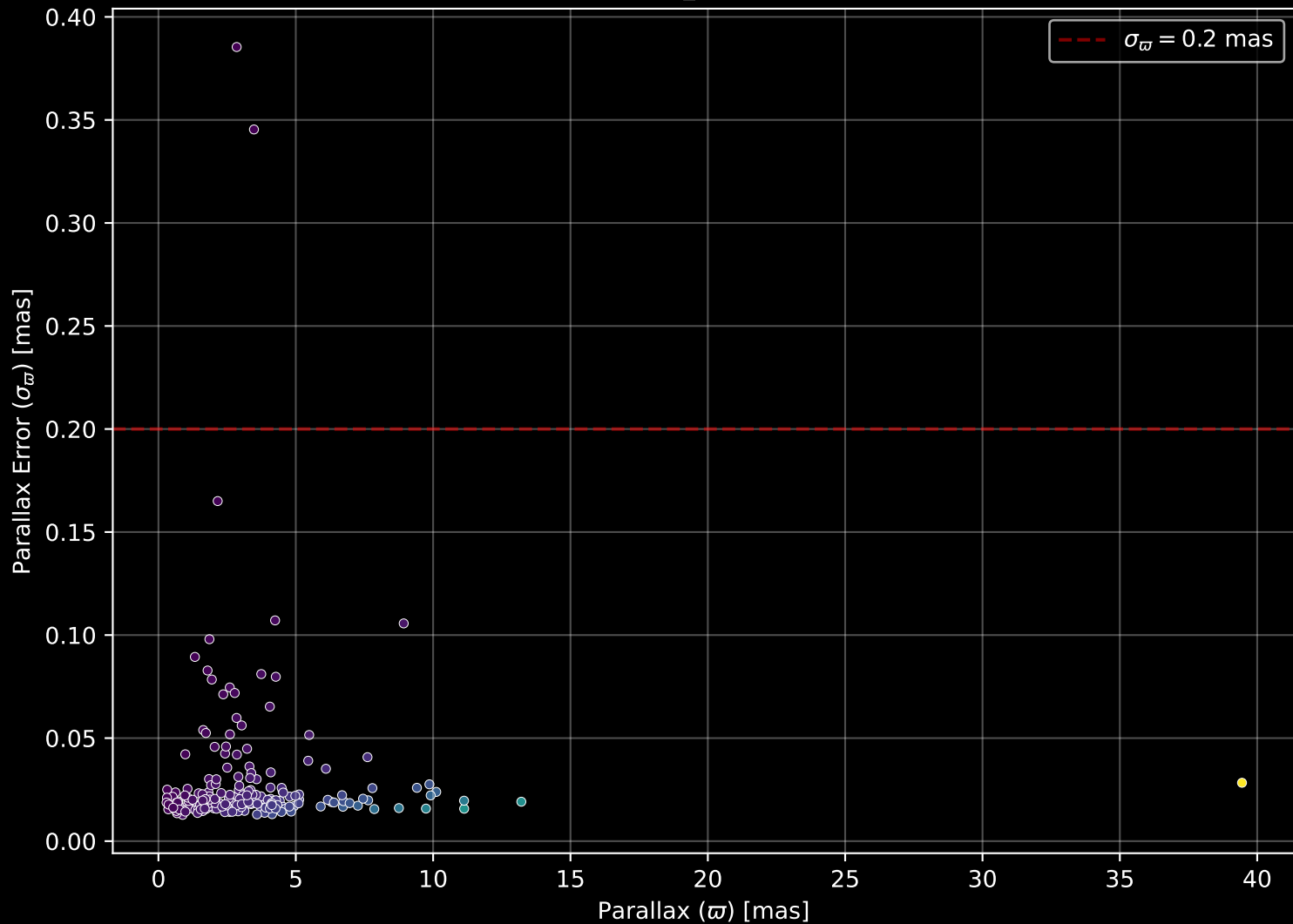
APOGEE DR17 Field: [171-52_MGA] Parallax Quality (n= 200)
